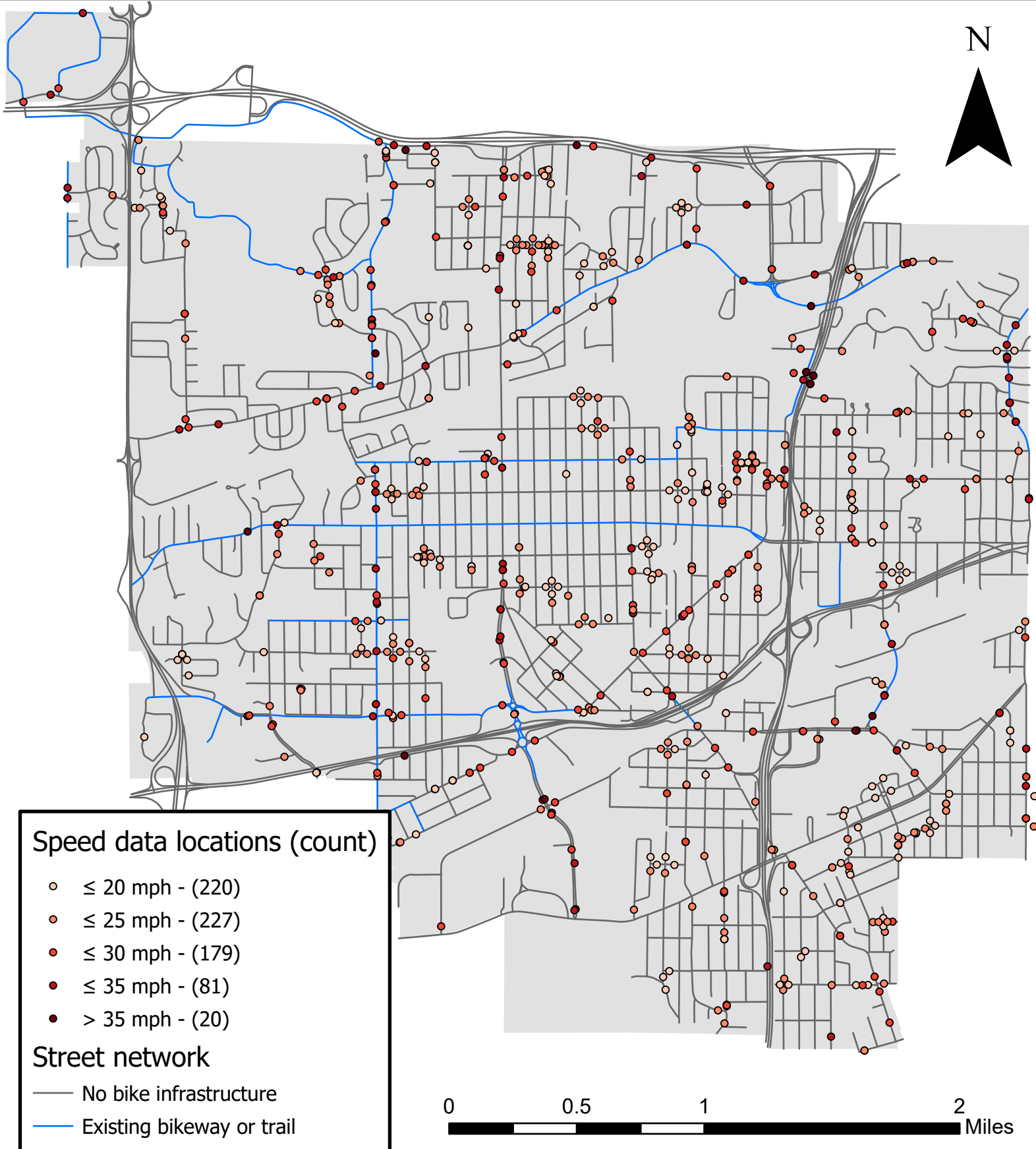
Fig 6: Average speeds on existing bikeways
