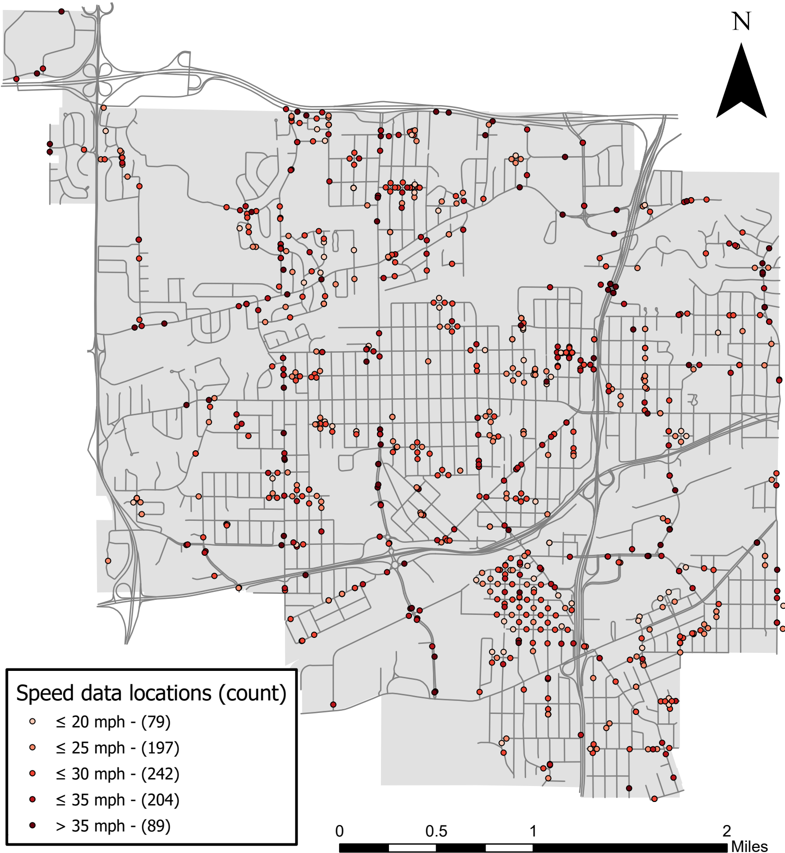
Figure 4: 85th percentile vehicle speed
